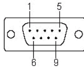
Figure 5.1: PCI-1601/1602 Pin Assignment
