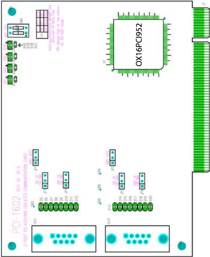
Figure 2.3: PCI-1602A/B Silk Screen
