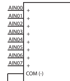
Grafik 6.1 A/D-Wandler Single-ended
